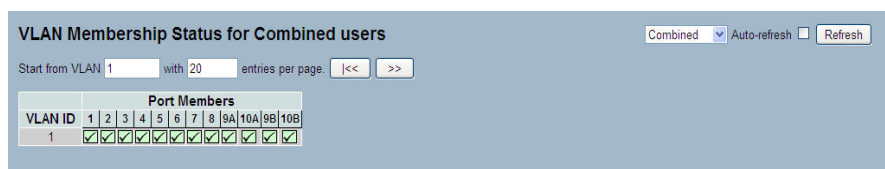
Figure 3-10.3: The VLAN Membership Status for Static user
