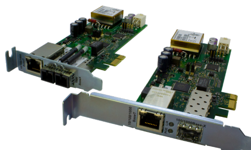
N-GXE-POE-xx-01 Series
