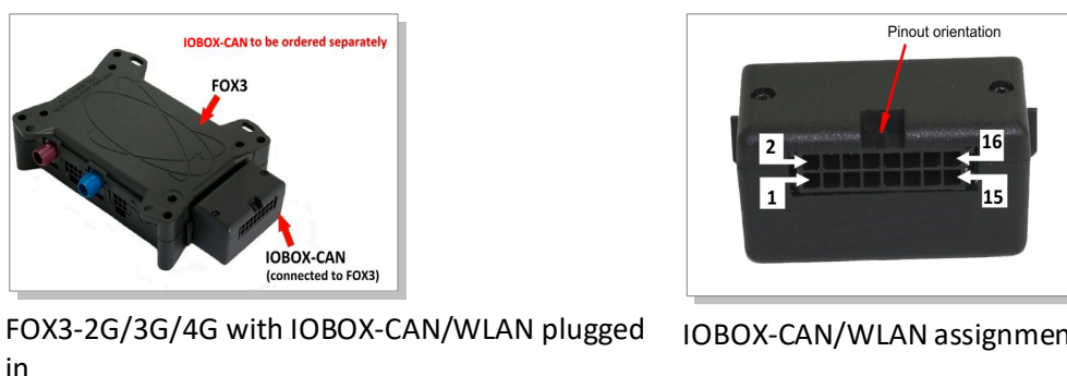
Figure 24: IOBOX-CAN/WLAN pinout.
