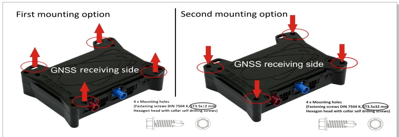
Figure 25: View of the mounting holes
