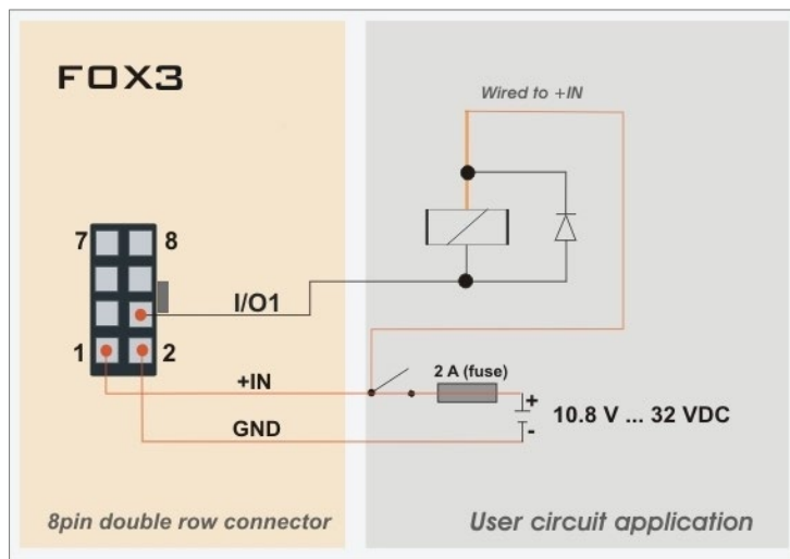
Figure 10: Connection example 1 when using it to control a Relay.
