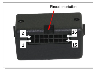
IOBOX-CAN/WLAN assignment
