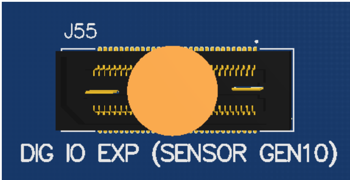
Figure 11 J55 Gen-10 Sensor Connector (Samtec QSH-030 series)
