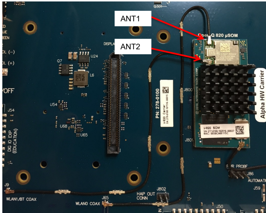
Figure 16 On Board PCB Antennas
