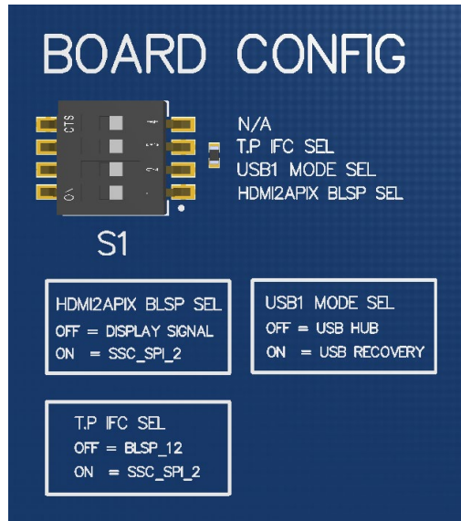
Figure 30 S1 Board Configuration Switch (on Bottom of Development Kit)
