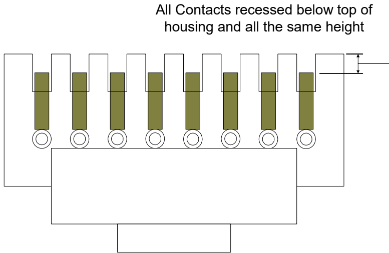
Good Crimp on wire Figure B
