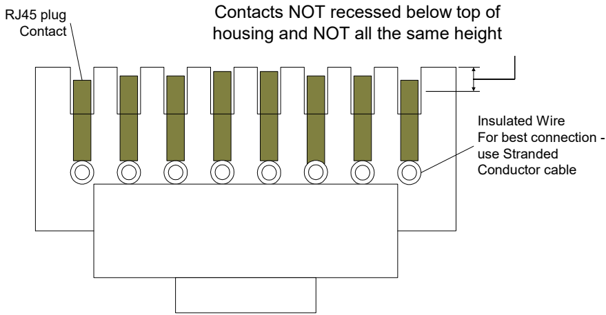
Bad Crimp on wire Figure A
