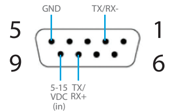
DB9F in RS485 (2-Wire) Mode
