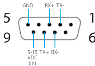
DB9F in RS422/485 (4-Wire) Mode
