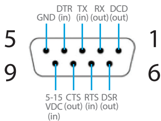
DB9F in RS232 Mode
