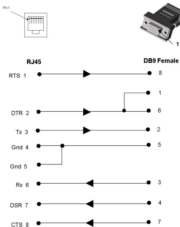
Figure C-4 RJ45 Receptacle to DB9F DCE Adapter for the SLB (PN 200.2070A)
