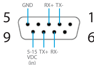
DB9F in RS422/485 (4-Wire) Mode (xDirect485 & PoE Models)
