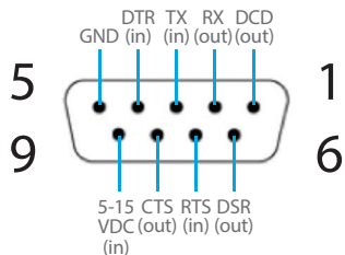
DB9F in RS232 Mode (All models)
