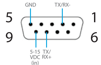
DB9F in RS485 (2-Wire) Mode (xDirect485 & PoE Models)
