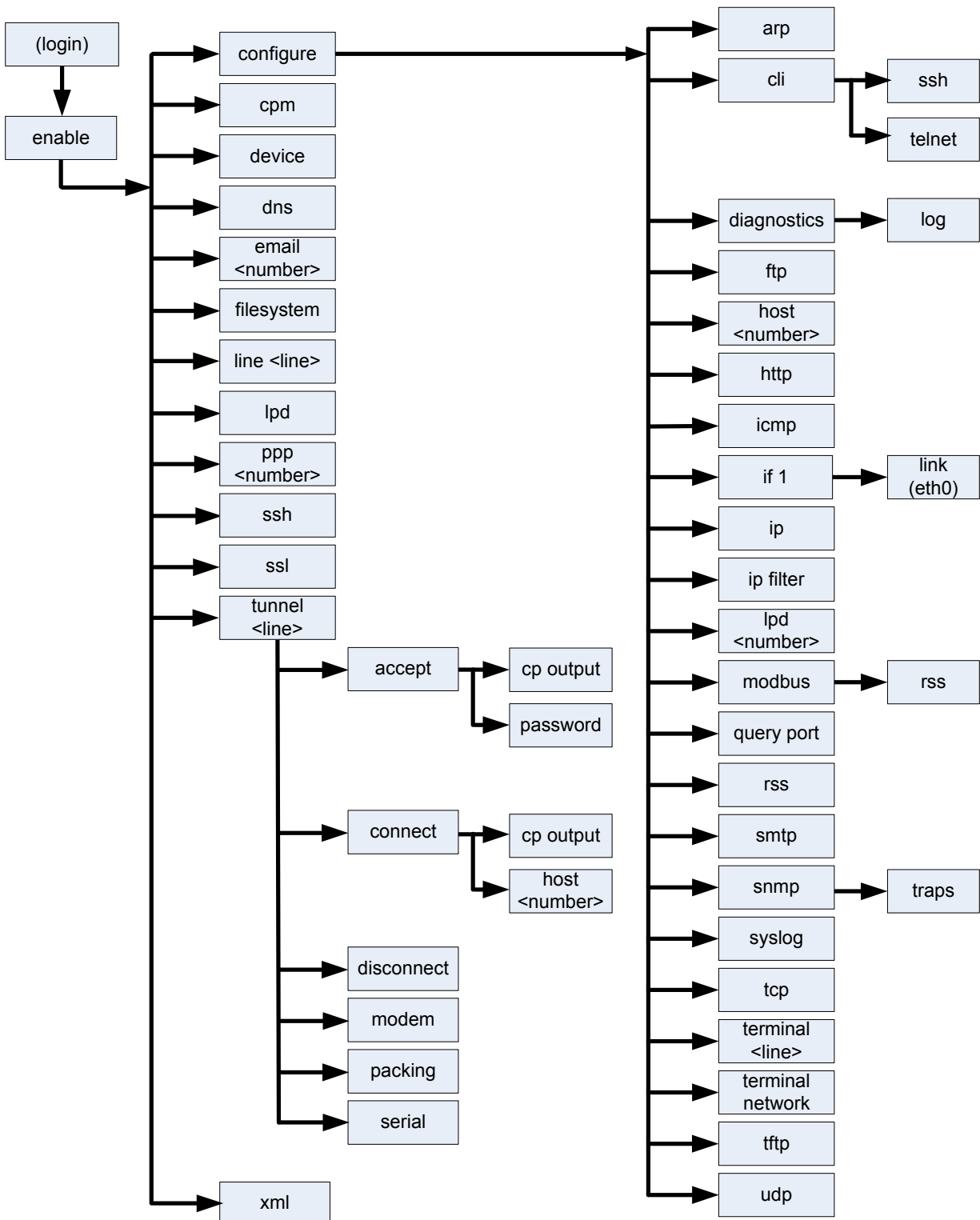
Figure 3-1 CLI Level Hierarchy
