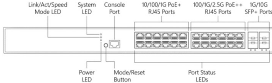
SM24TBT4XPA Front Panel
