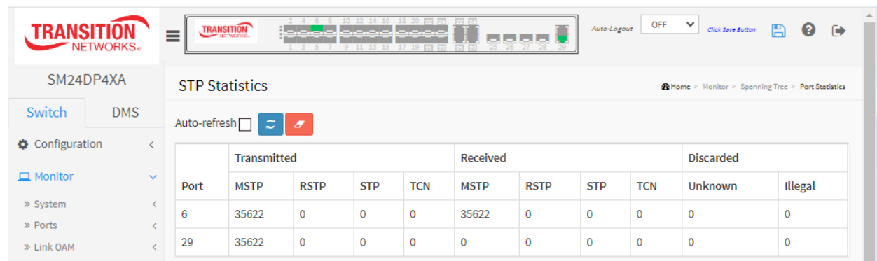
Figure 3-8.3: STP Statistics
