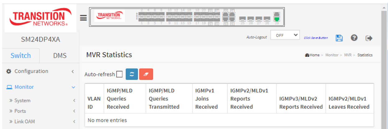
Figure 3-10.1: MVR Statistics
