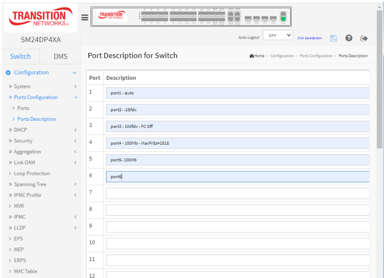
Figure 2-2.1: Port Description for Switch
