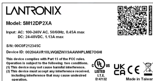
Device Label
