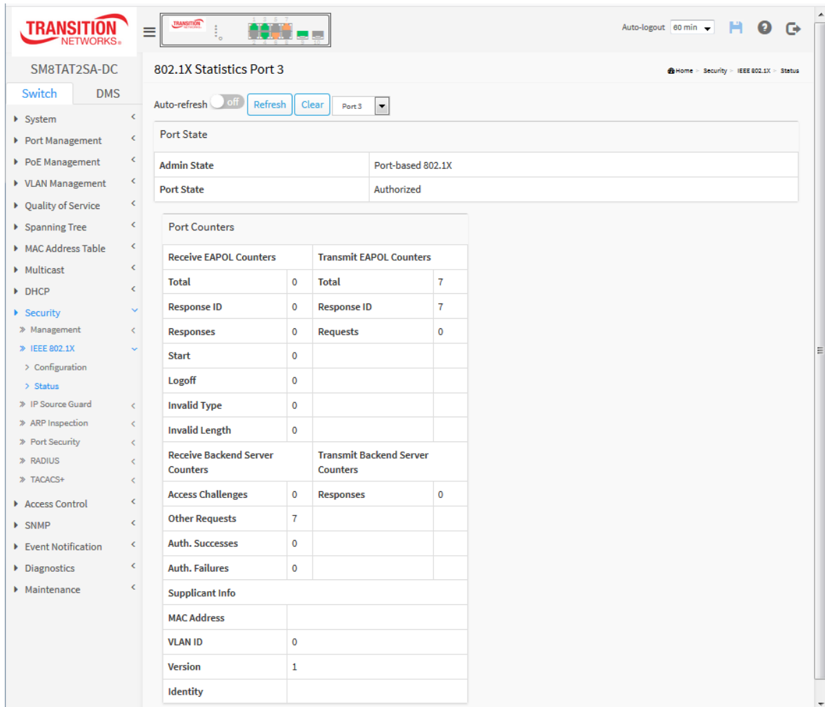
Figure 12-2.2: 802.1X Statistics
