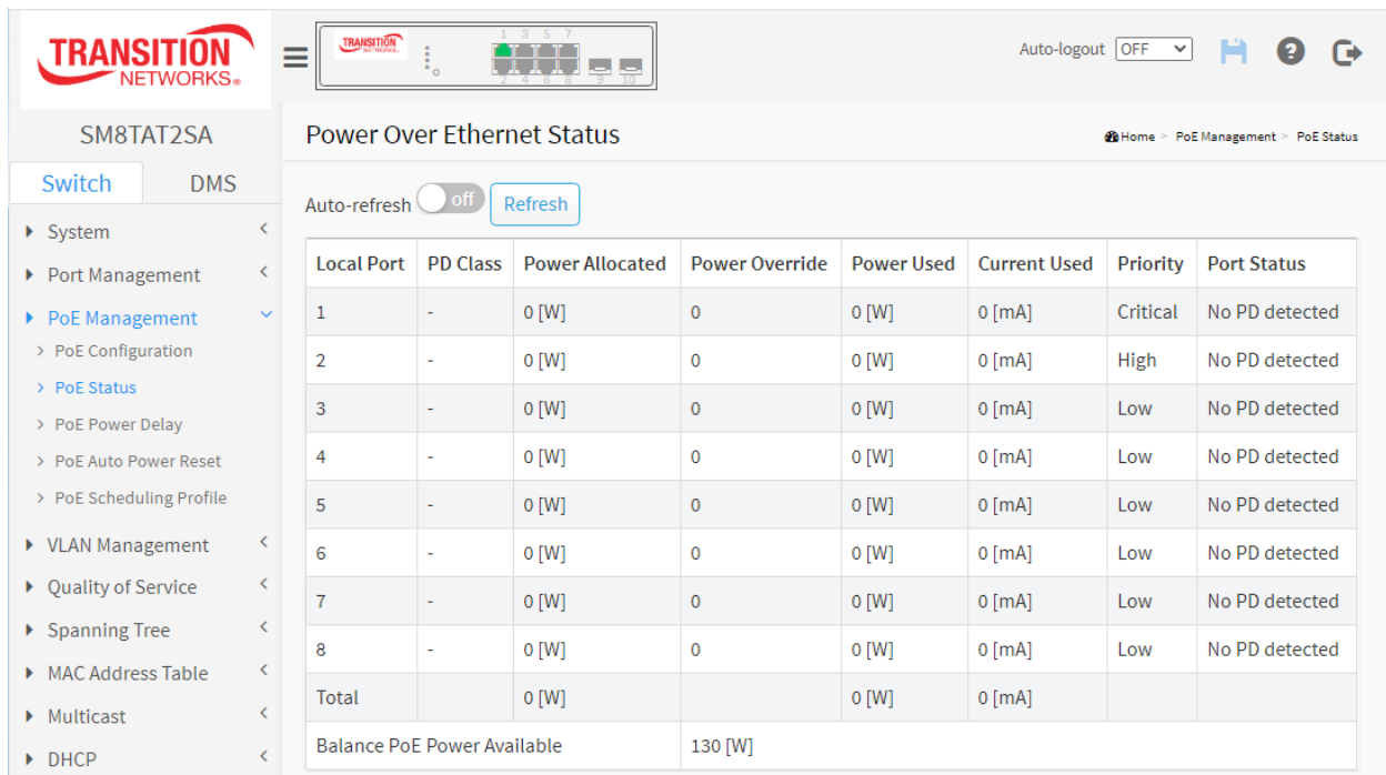
Figure 5-2: PoE Status
