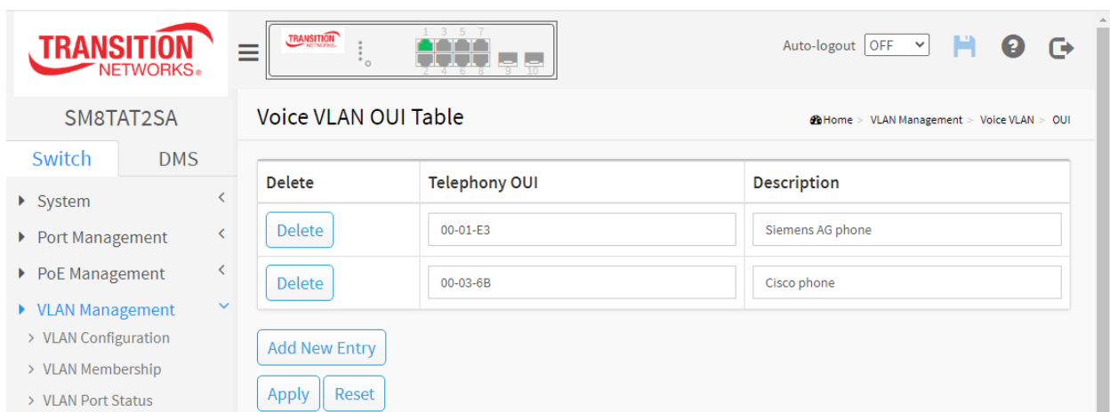
Figure 6-6: Voice VLAN OUI Table
