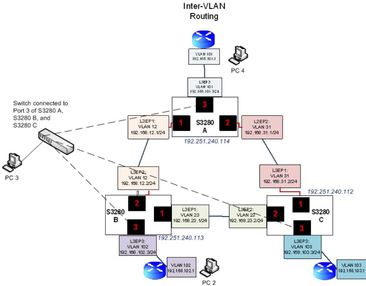
Figure 6. InterVLAN Routing Setup Example
