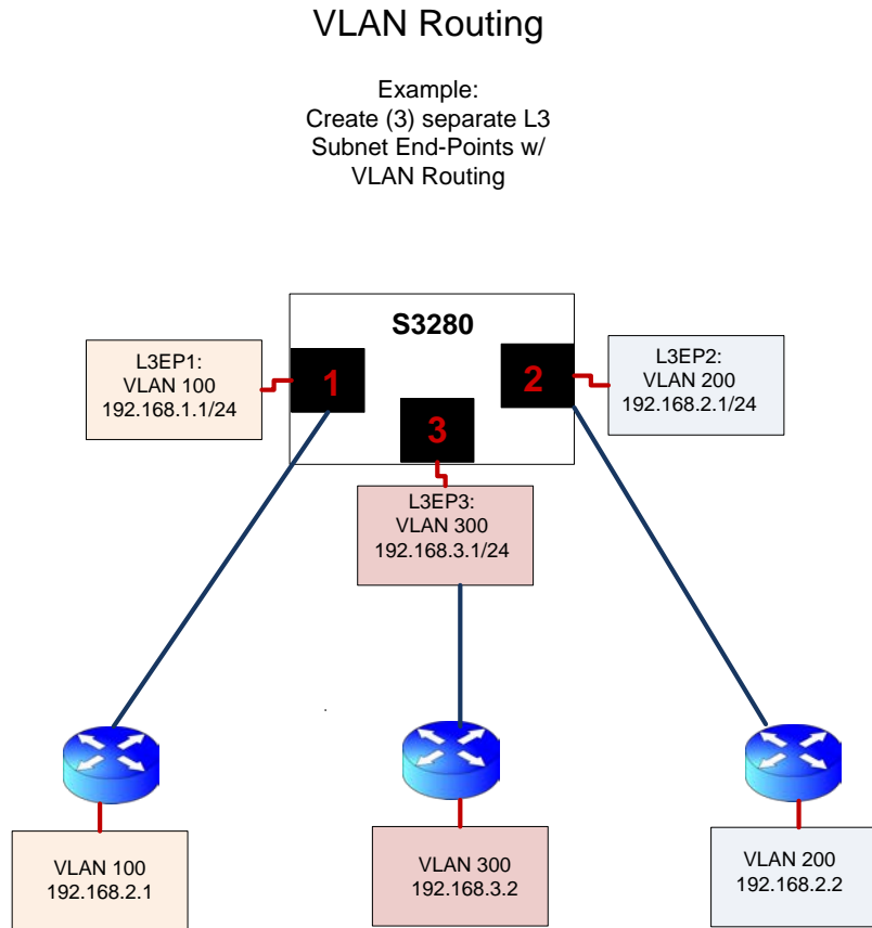
Figure 5. VLAN Routing Setup Example
