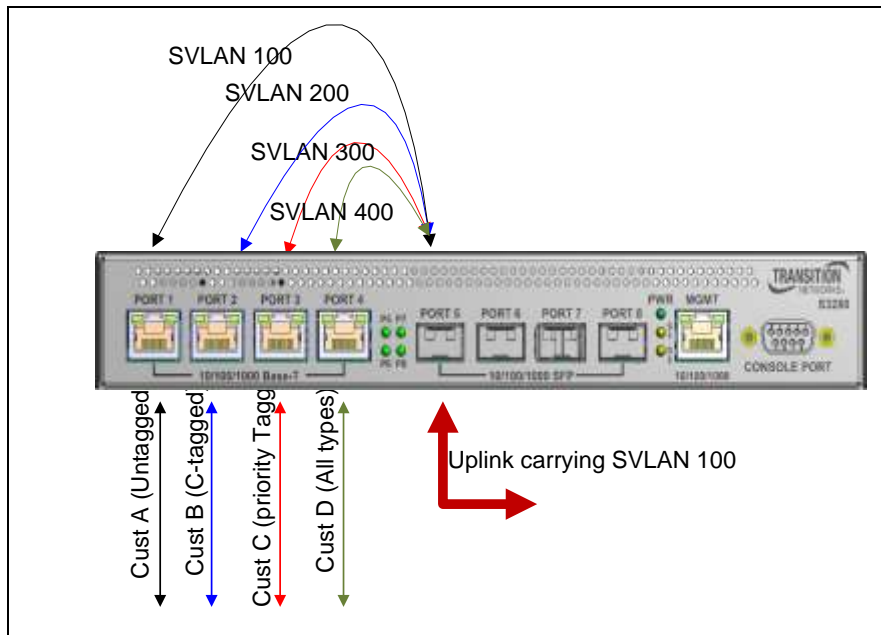
Figure 14. S-VLAN with one trunk (Multiple UNI bundled at the Operator domain)
