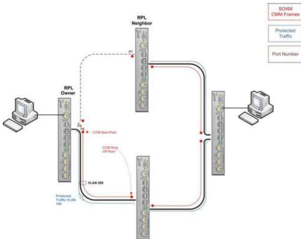
Figure 4. ERPS Example
