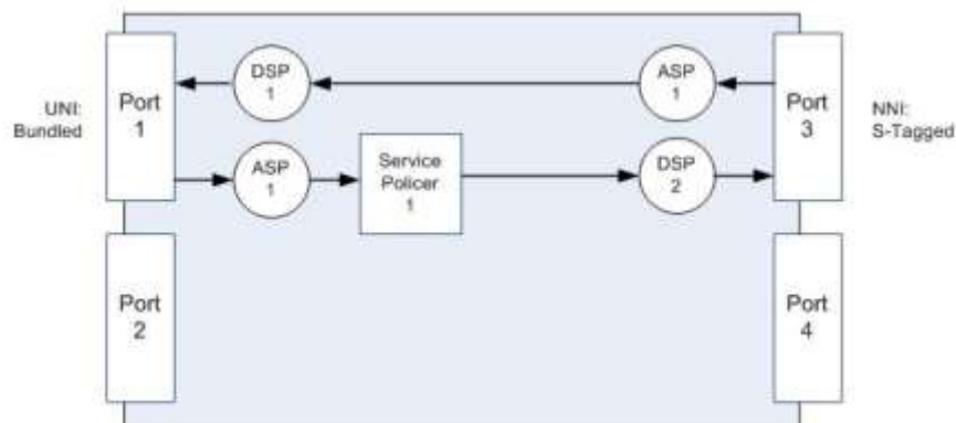
Figure 21. Provider Bridge E-LINE Service
