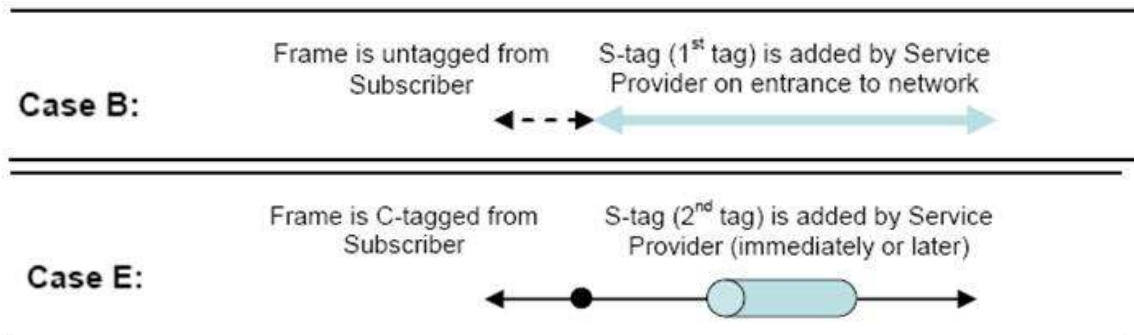
Figure 12. All to one bundling VLAN Cases
