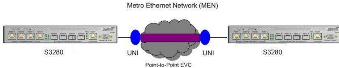
Figure 15. EPL service per MEF 6.1
