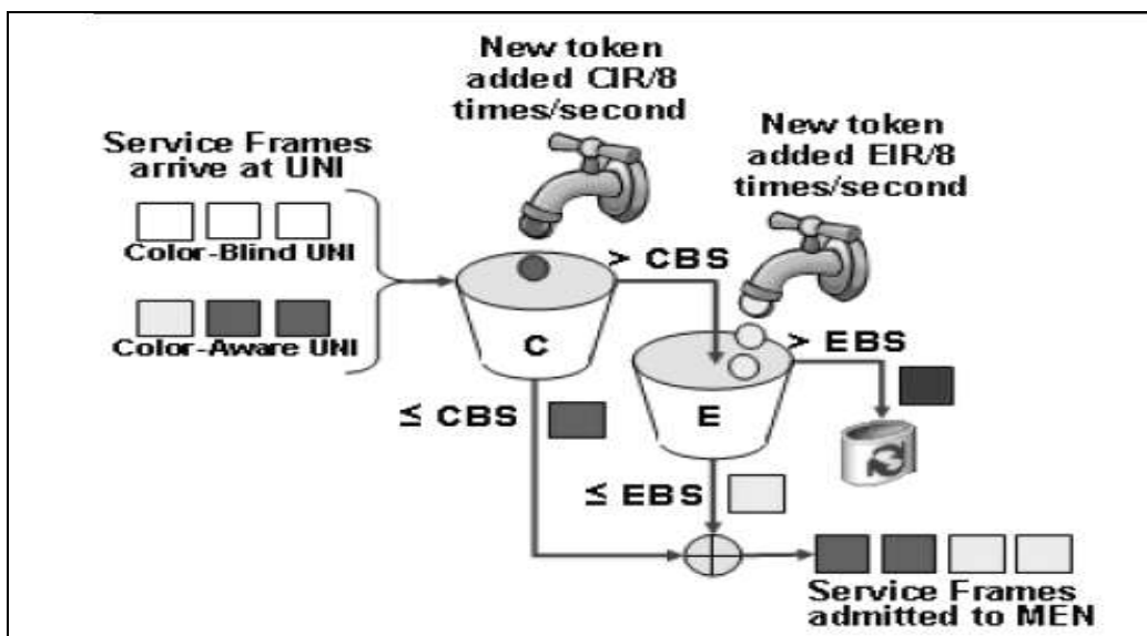
Figure 22. Color Aware Dual leaky bucket for Bandwidth Profiling
