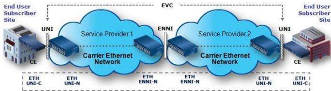
Figure 20. Provider Bridge E-LINE Service
