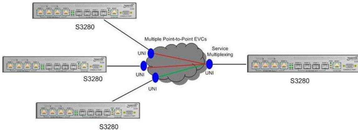
Figure 16. EVPL Service per MEF 6.1
