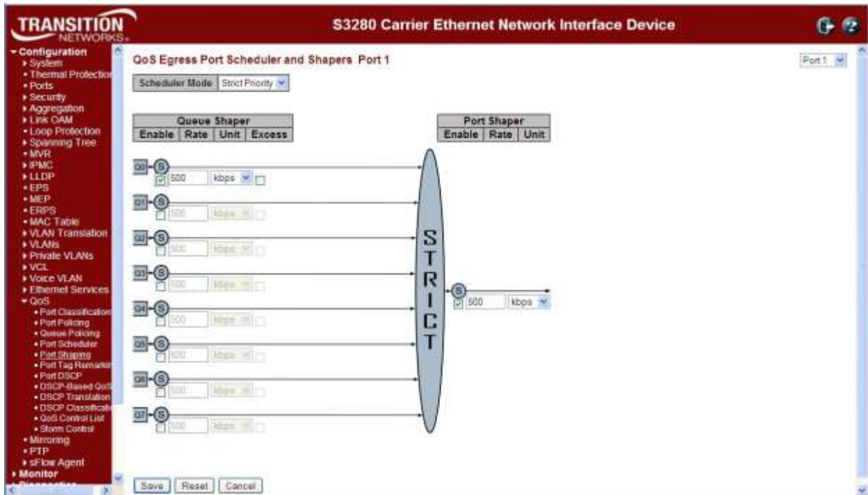
Figure 24. Egress Shaper on Port 1
