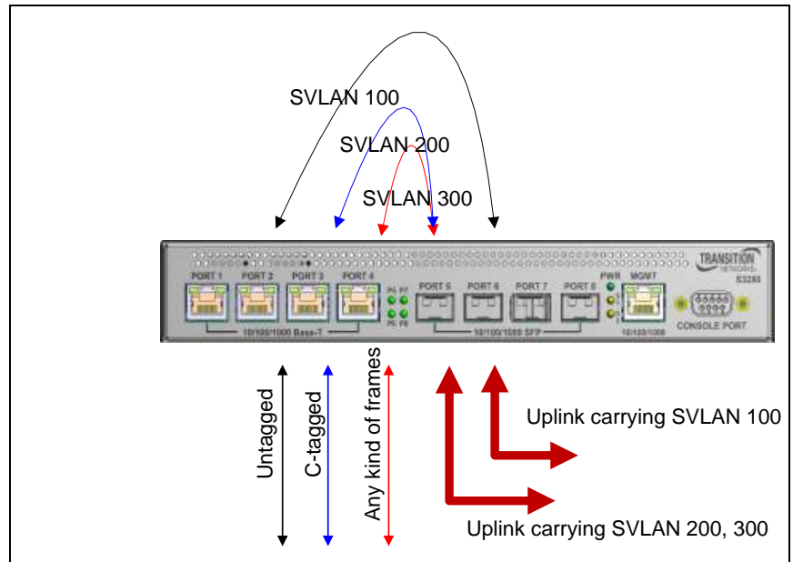
Figure 13. S-VLAN with multiple trunks (EPL service at 3 different UNIs)
